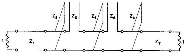
Fig. 6. Seven-section filter containing unit elements and stubs [3]. All sections are quarter-wave at 2.175 GHz.
